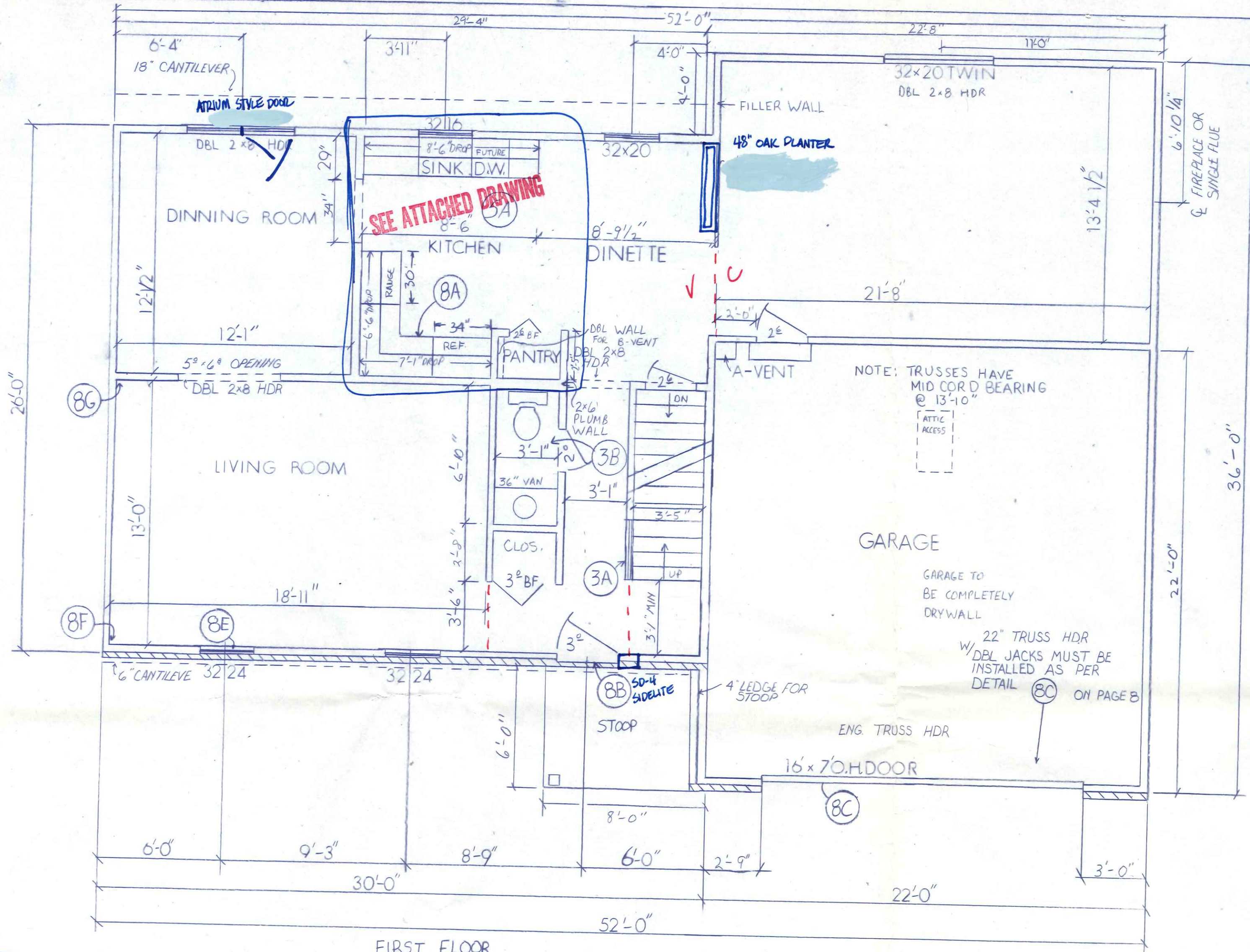
FIRST FLOOR
