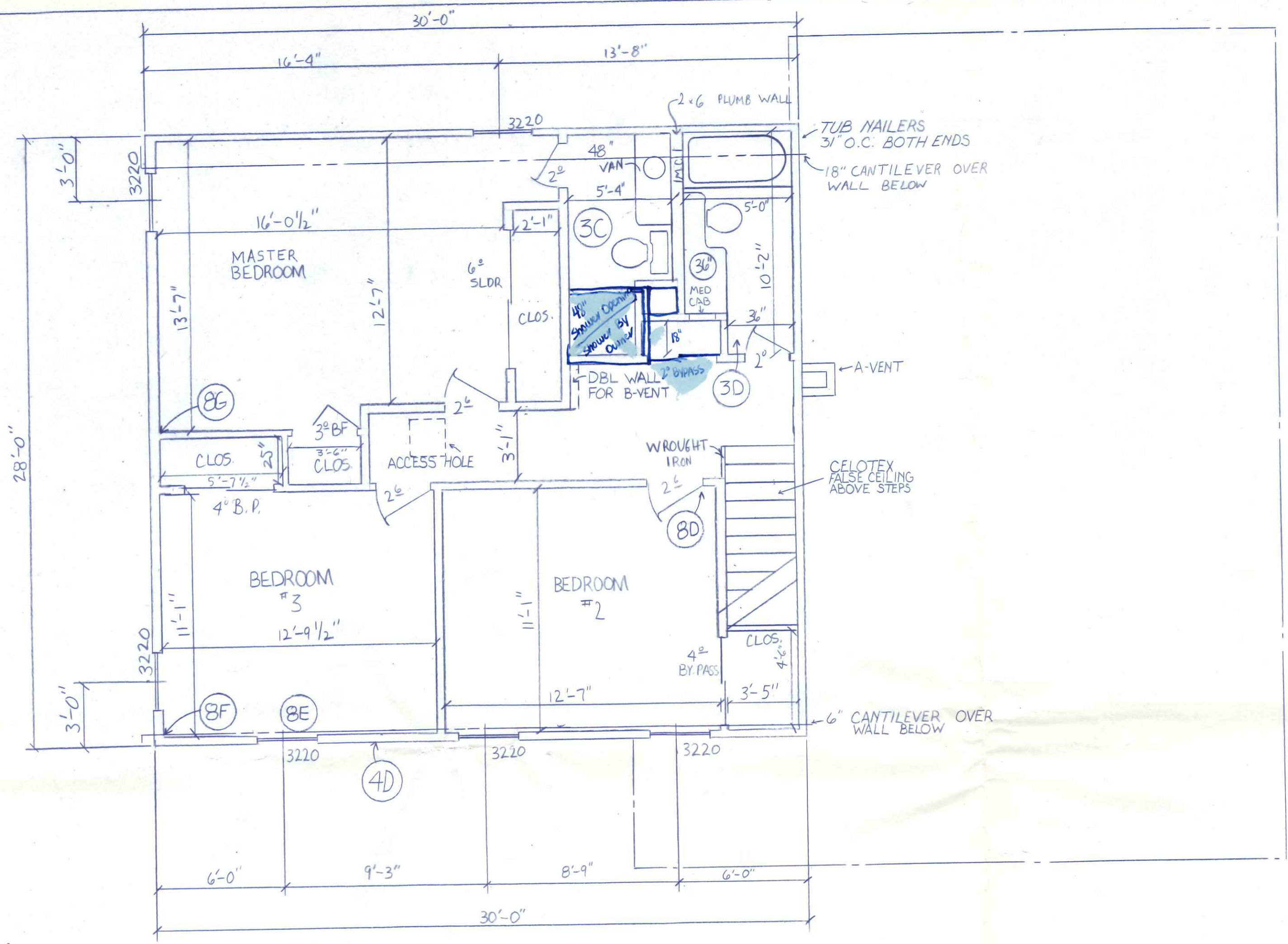
SECOND FLOOR
